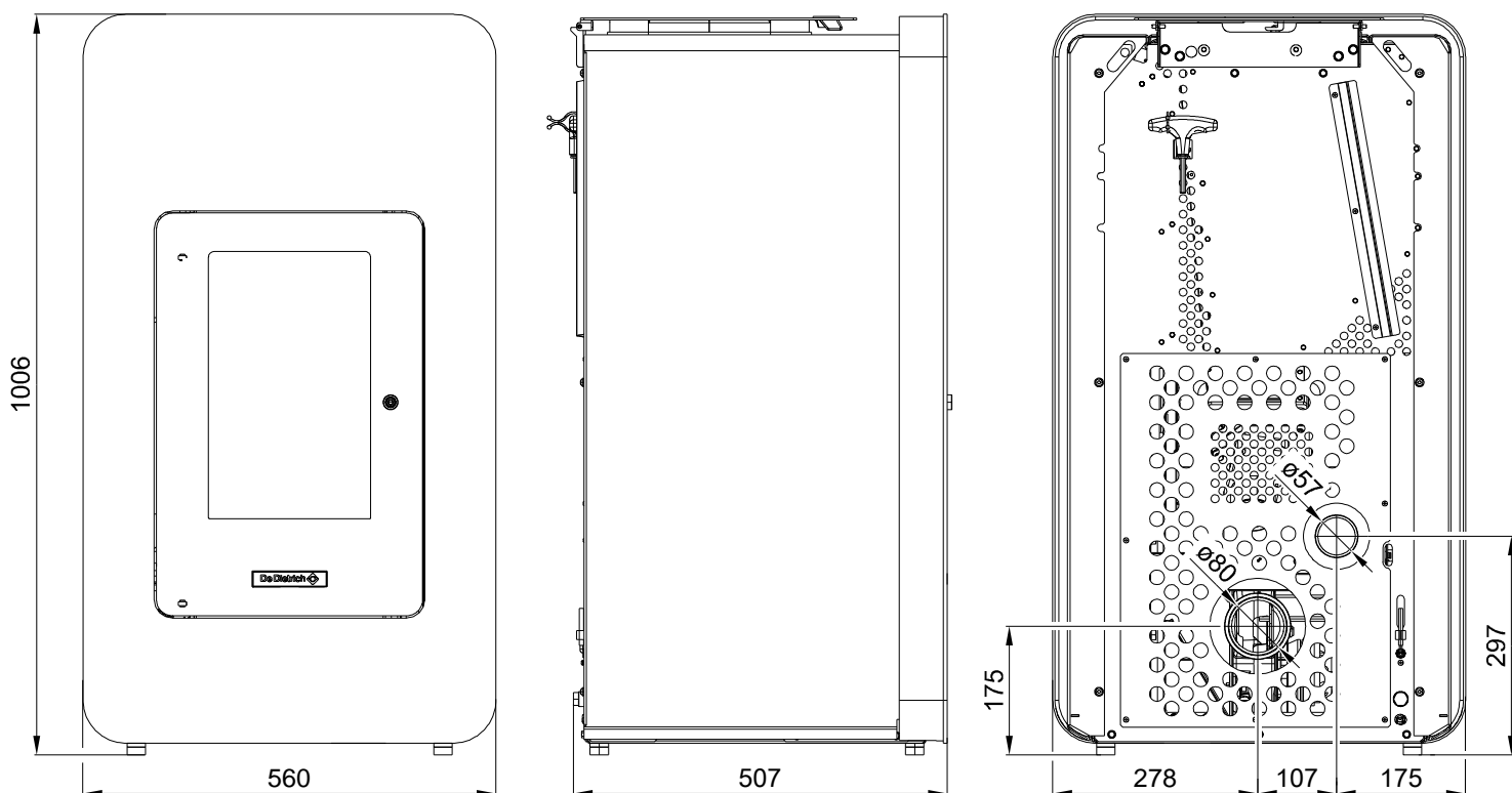
Illustration 19 : Quadralis PPA 8 BC
