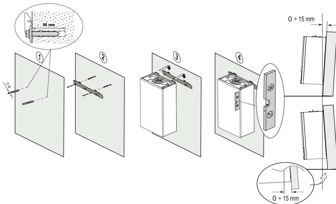
Fig.18 Installation murale
