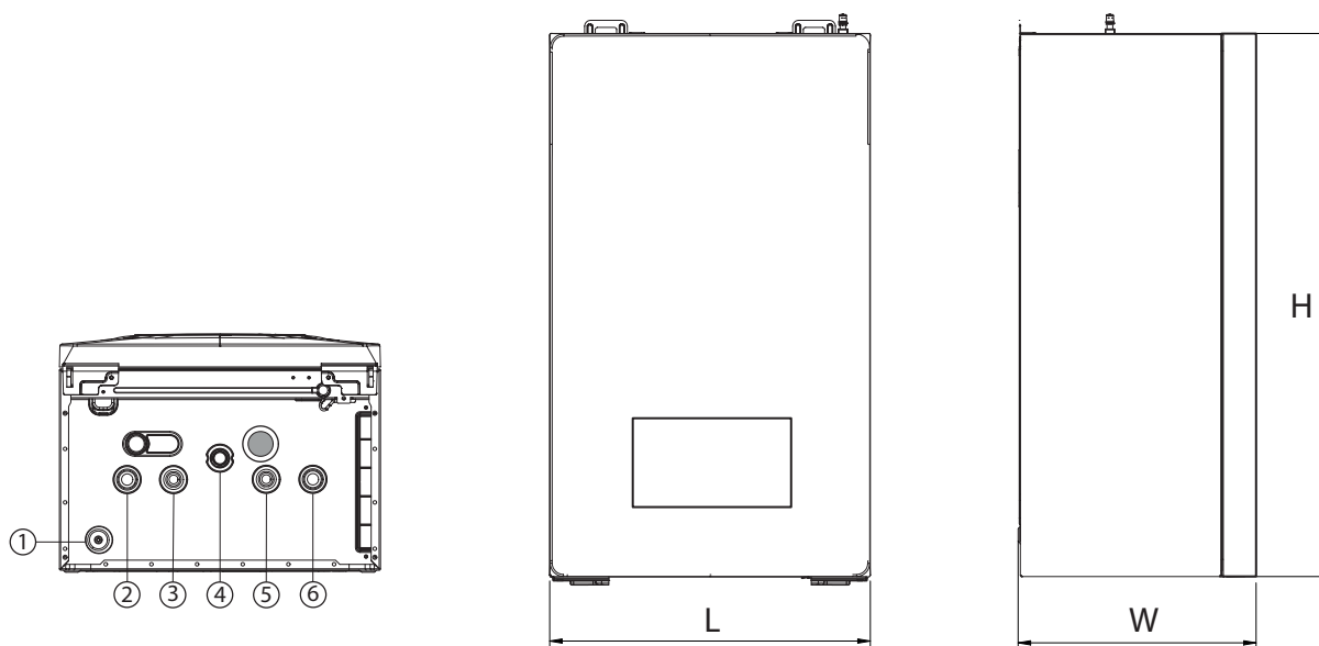
Fig.1 Dimensions et raccordements
