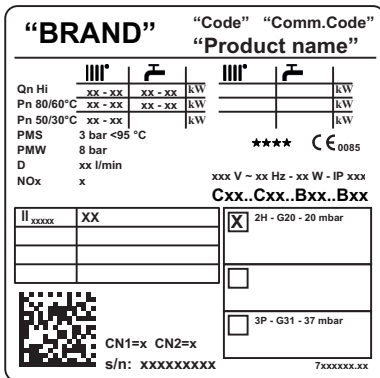
Fig.15 Plaque signalétique
