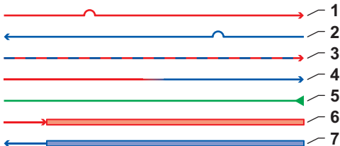
Fig.80 Tubage
