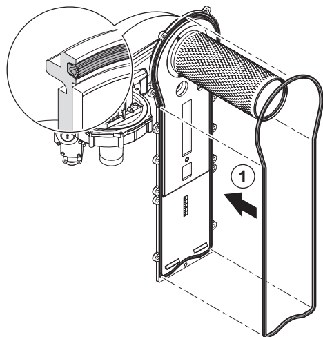
Fig.120 Montage du joint
