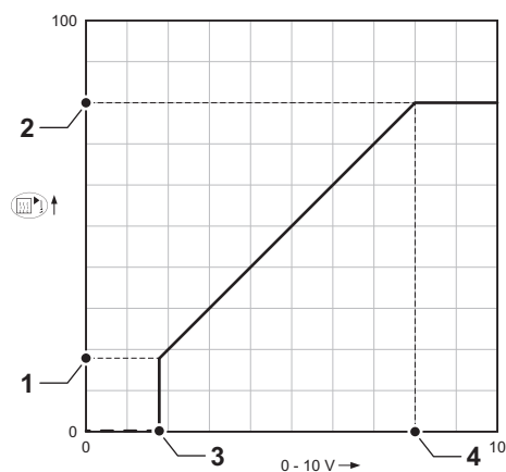
Fig.78 Commande 0-10 V
