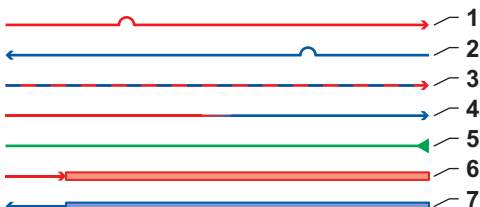
Fig.27 Tubage
