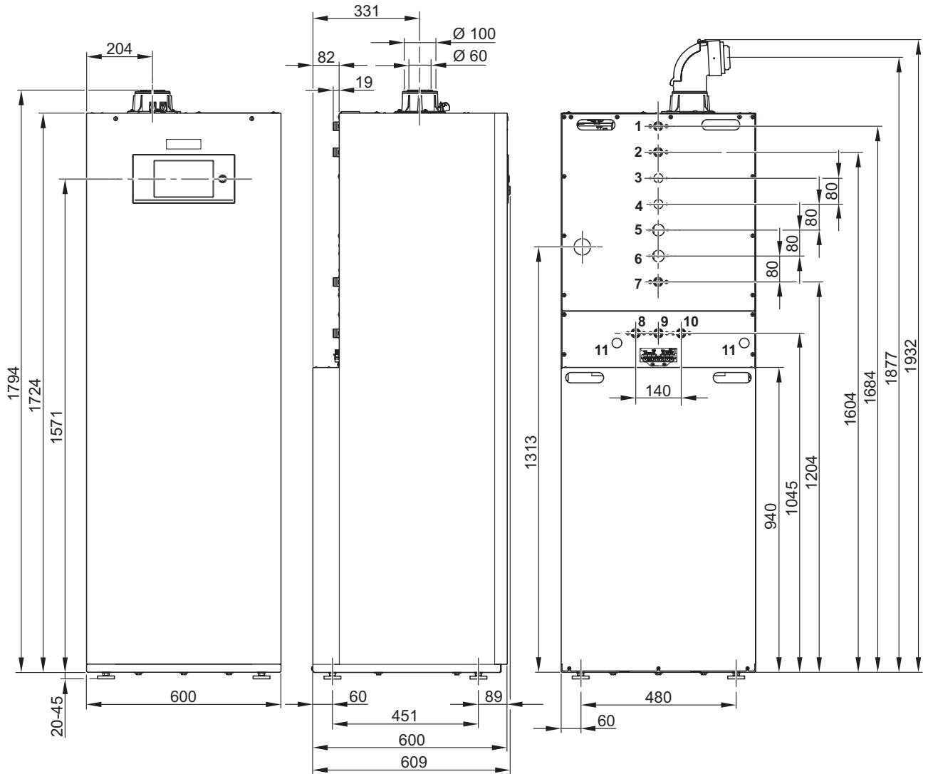
Fig.2 Dimensions et raccords EGC EVO
